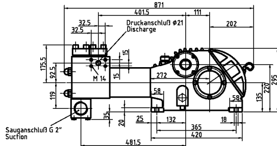
Niederdruckkopf MC Compact Head (Low Pressure) MC
